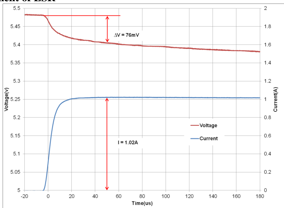
Fig 3: Measurement of ESR for an HW203
