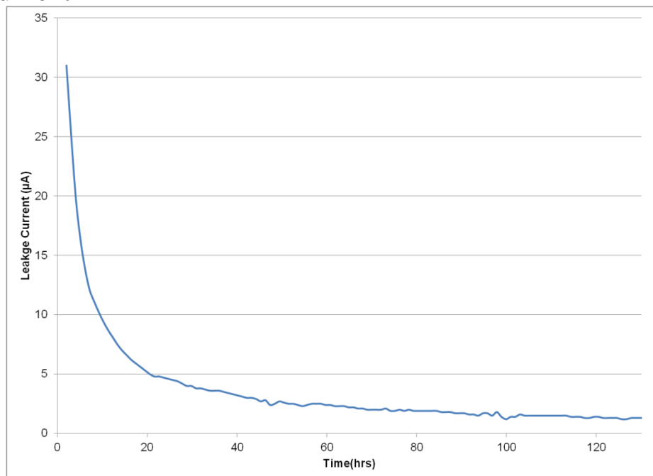
Fig 10: Leakage Current
