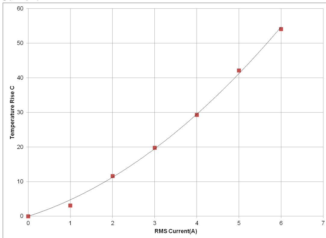
Fig 12: Temperature rise in HW203 with RMS current
