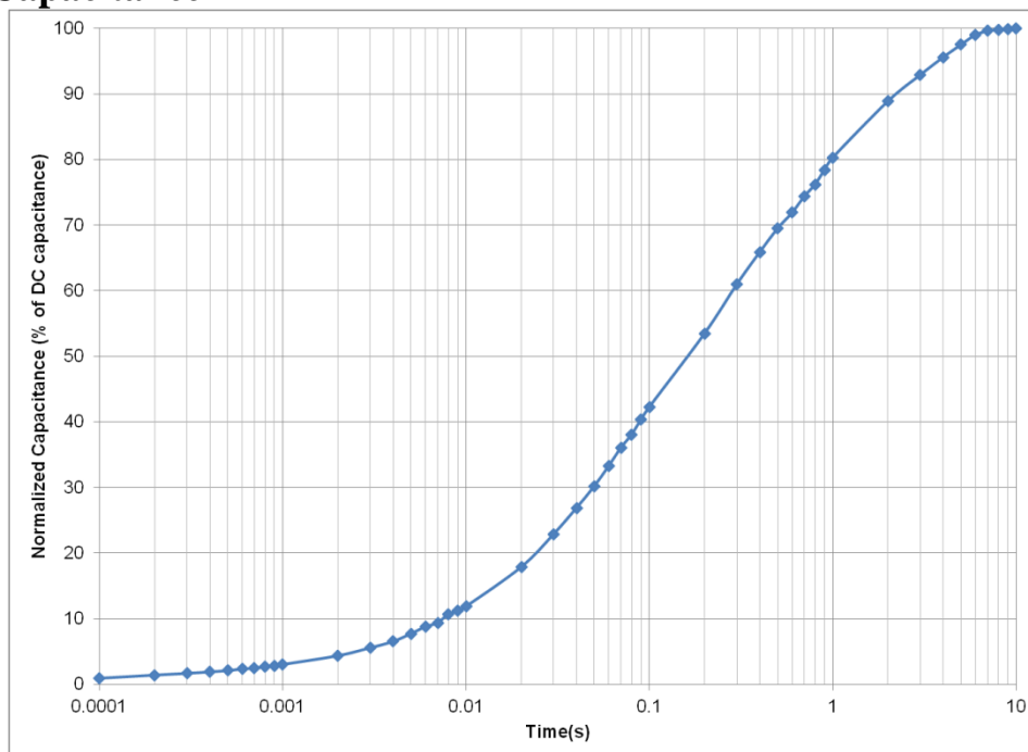
Figure 4: Effective Capacitance
