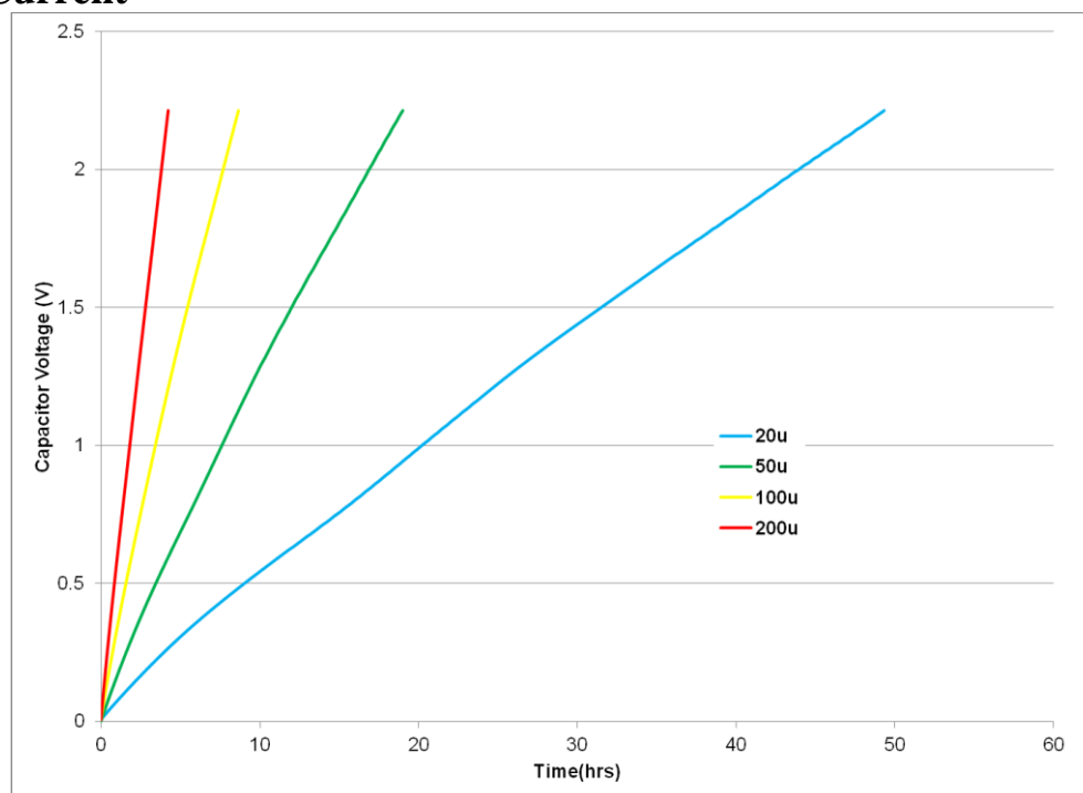
Fig 11: Charging an HW103 with low current
