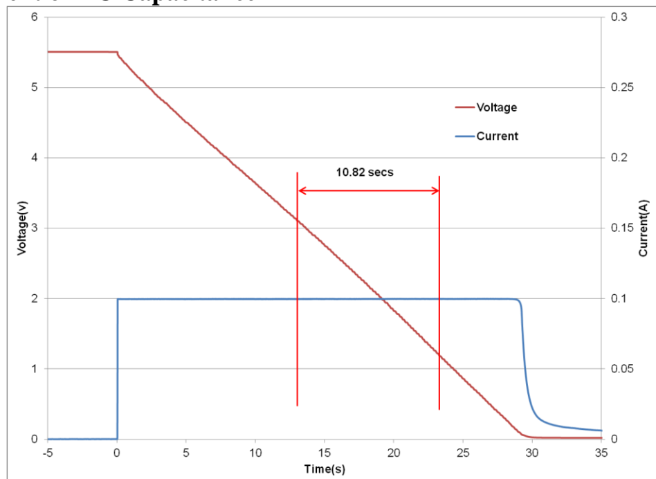
Fig 2: Measurement of DC Capacitance for an HW203
