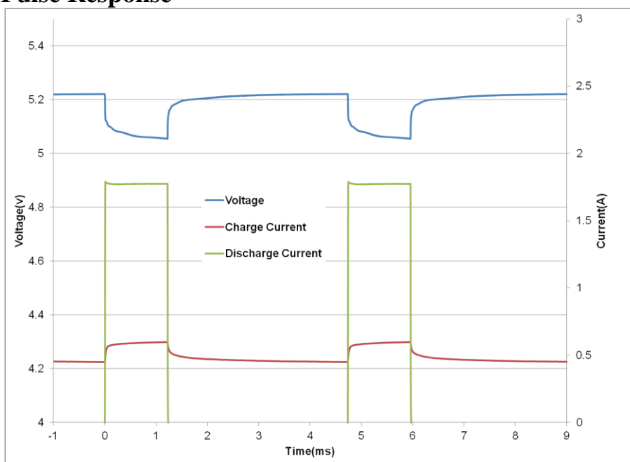
Fig 5: HW203 Pulse Response with GPRS Class 10 Pulse Train
